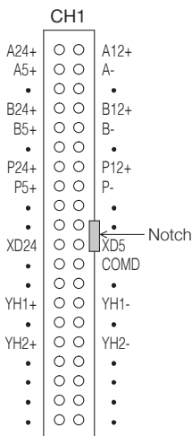
FX3U-32DP
