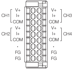
FX5-4AD
