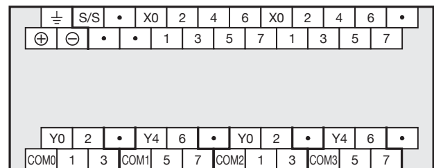
FX5-32ET/DSS
