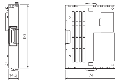
FX5-CNV-BUSC
