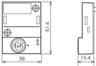
FX5-422-BD-GOT
