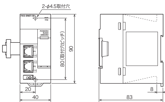
FX5-ENET/IP
