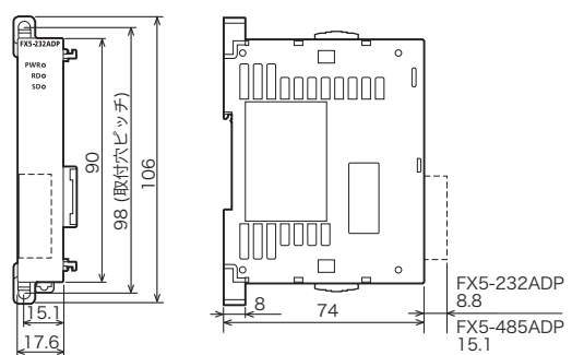
FX5-232ADP / FX5-485ADP
