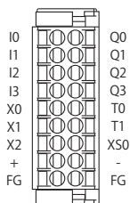
FX5-SF-MU4T5
