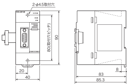
FX5-DP-M
