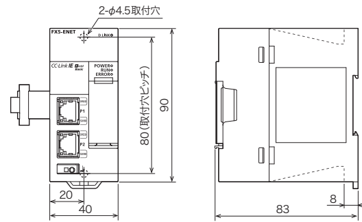
FX5-ENET
