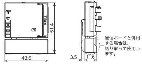
FX5-SDCD
