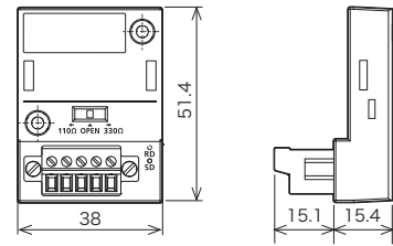
FX5-SDCD
