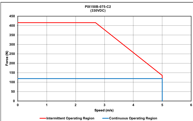
PIX150B-075-C2
