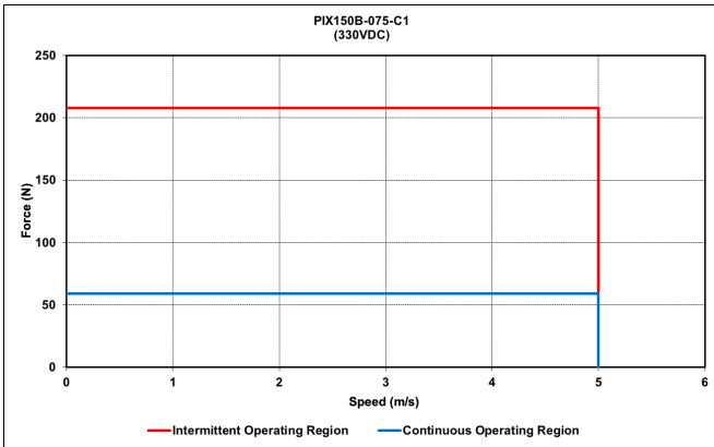
PIX150B-075-C1
