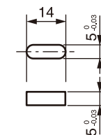
Accessory sunk key
