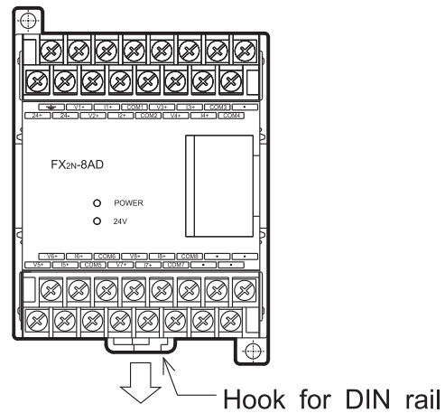
Figure 4.1: Installation with DIN rail
