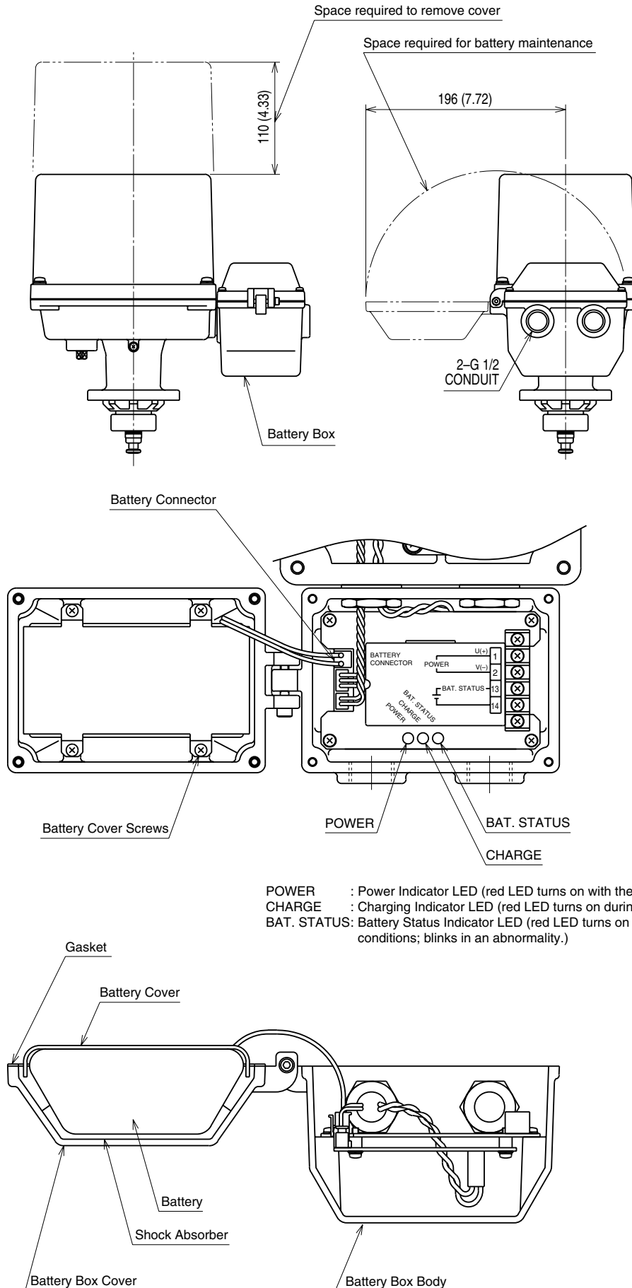
Figure 1. Component Identification
