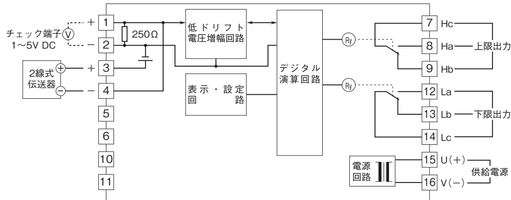
■48NAVD-2 (2点警報/2接点出力)
