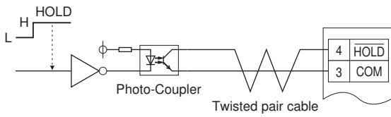
(a) Photo-Coupler
