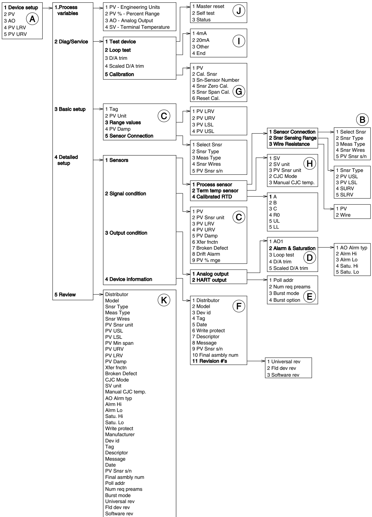
Figure 1. 27HU/27HU-B HART Communicator Menu Tree
