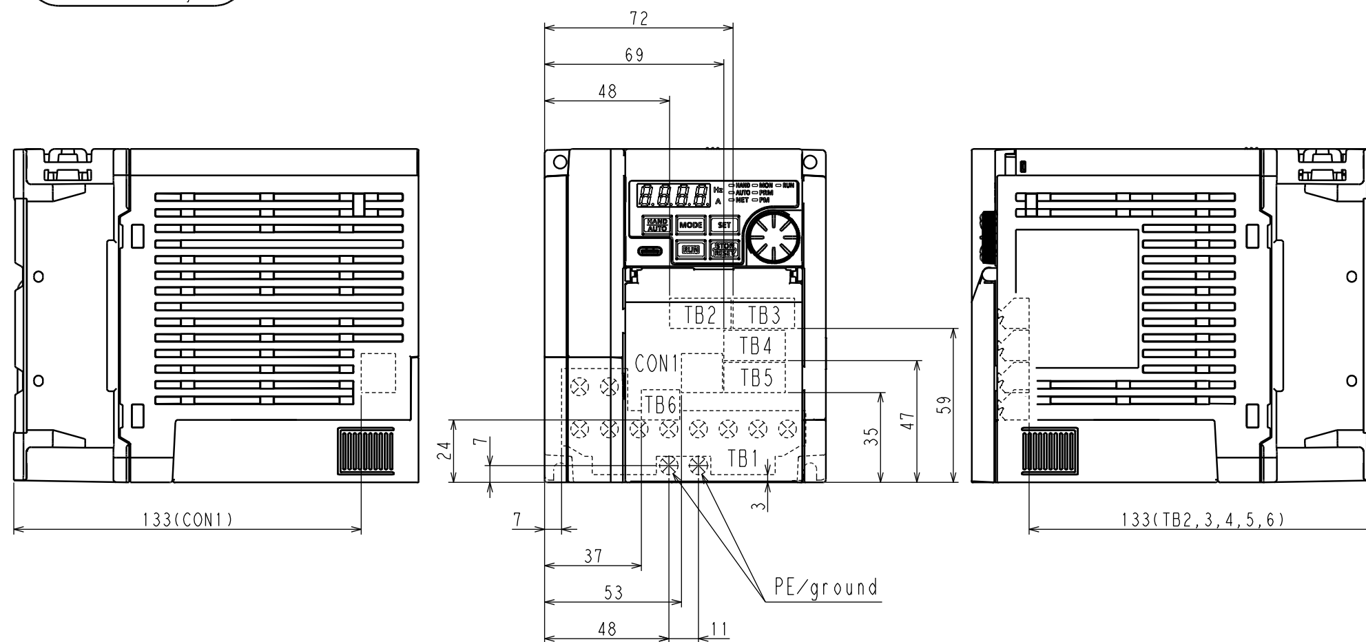
端子台配置 Terminal block layout
