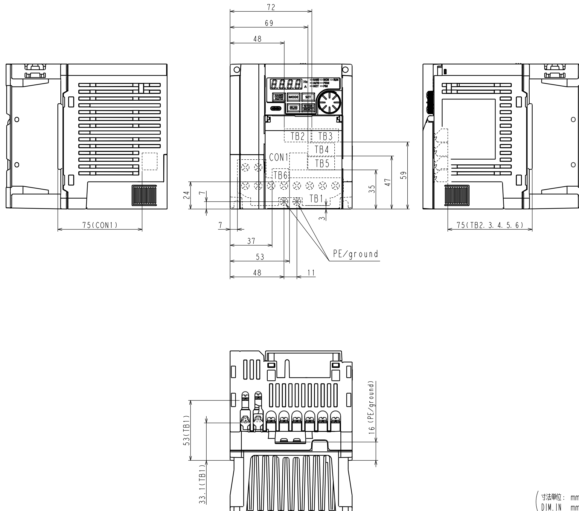
端子台配置 Terminal block layout
